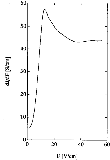
FIG. 10. Differential conductivity dj/dF vs electric-field strength for the parameters of Fig. 5.
