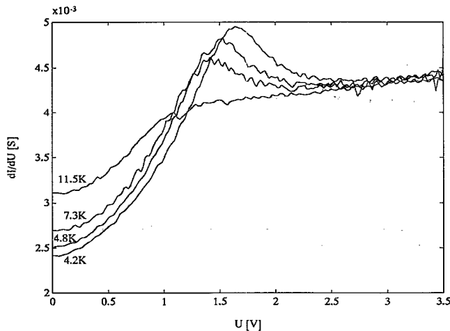
FIG. 5. Temperature dependence of \sigma_{\text{diff}} for sample A as a function of the voltage.
