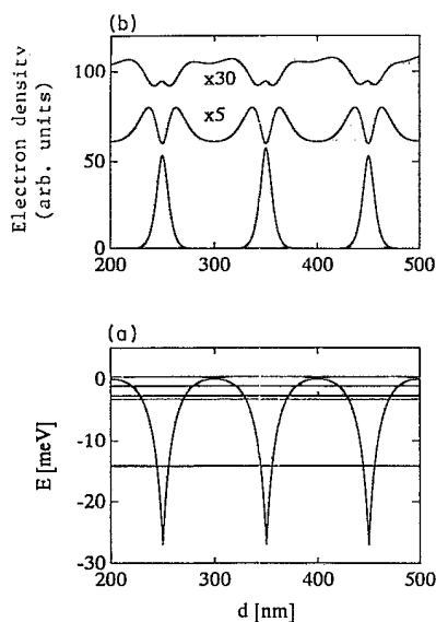
FIG. 1. (a) Conduction-band edge of sample A . (b) Electron densities in the zeroth, first, and second subbands.
