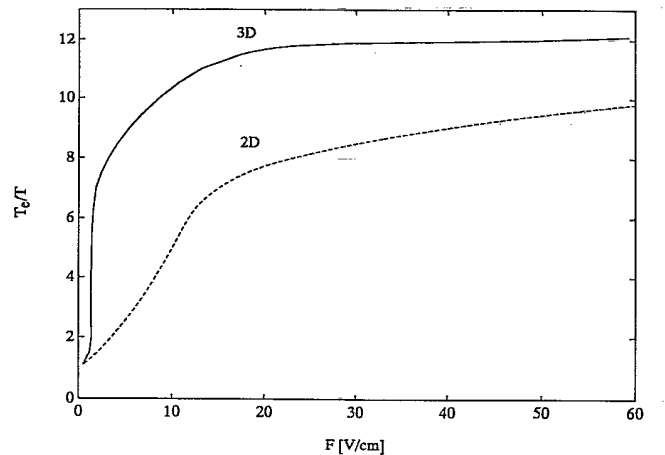
FIG. 7. Electron temperatures vs electric-field strength.
