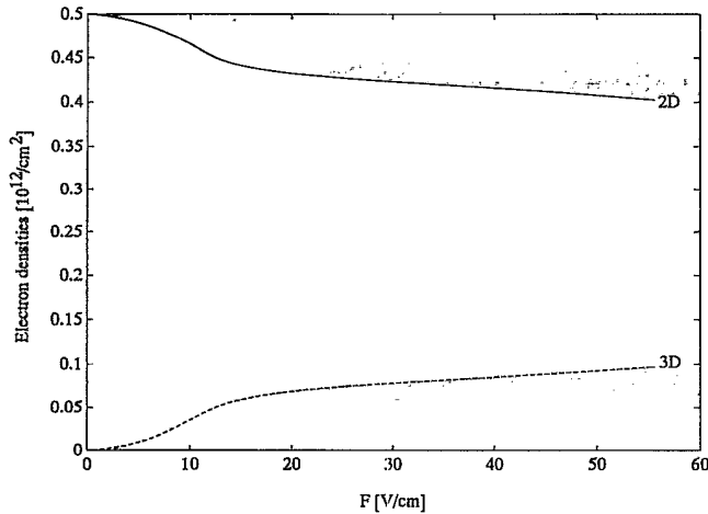
FIG. 8. Field dependence of the 2D and 3D carrier densities.
