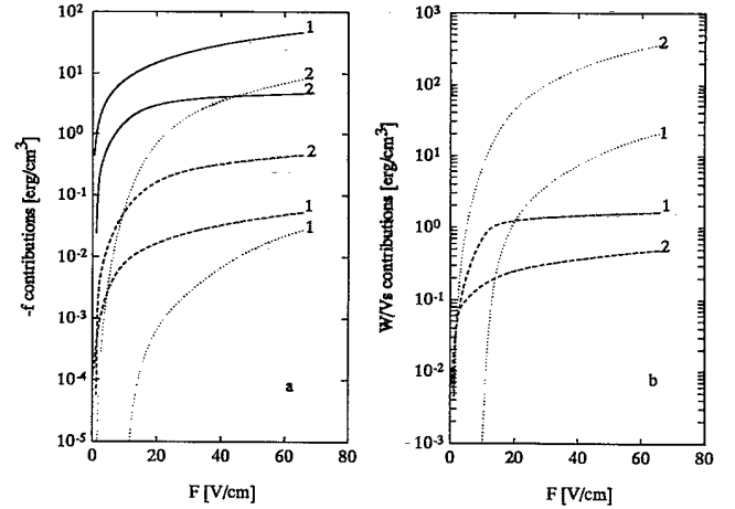
FIG. 6. (a) Friction forces as functions of electric-field strength for momentum relaxation on ionized impurities (solid lines), acoustic phonons as the sum of deformation and piezoelectric scattering contributions (dashed lines), and polar optical phonons (dotted lines). The data for the superlattice approximation are given in the text. (1) and (2) are the 2D and 3D parts, respectively. (b) Energy losses as functions of the electric-field strength.
