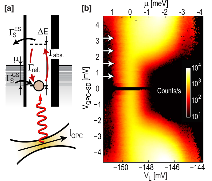
FIG. 3. (Color online) (a) Energy level diagram describing the absorption process. The electron in the QD is excited due to photon absorption, which allows it to tunnel out to the lead. (b) Quantum dot excitations, measured versus QPC bias voltage. The main peak at \mu=0 is due to equilibrium fluctuations between the source lead and the QD. As the gate voltage V_L is increased, the electrochemical potential of the QD drops below the Fermi level of the lead and only tunneling processes involving QD excitations become possible. Photon absorption is only possible for QPC bias voltages higher than the QD level separation \Delta E , giving rise to the shoulder-like features appearing at high V_{\text{QPC}} . The data was extracted from QPC conductances traces taken at G_{\text{QPC}} = 0.4 \times 2e^2/h , filtered at 50 kHz. The data taken at low QPC bias |V_{\text{QPC}}| < 0.4 \text{ mV} was filtered at a lower bandwidth (15 kHz) to allow counting in this regime.
