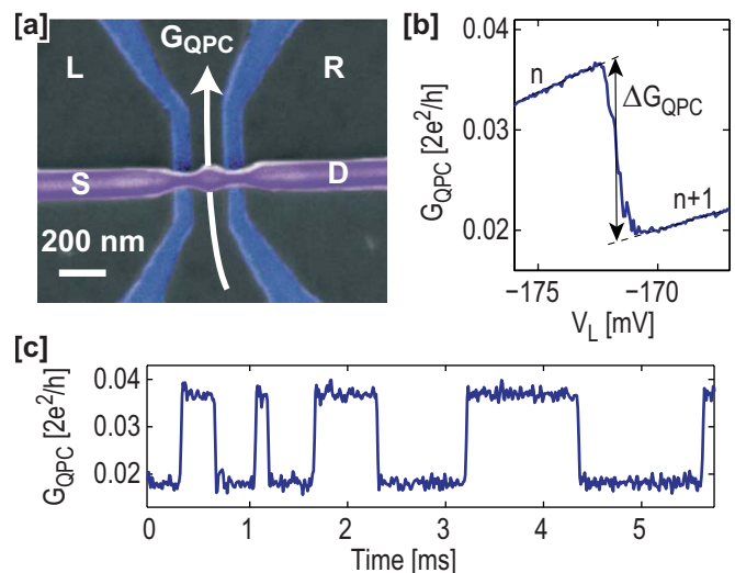
FIG. 1. (Color online) (a) SEM image of the device. The quantum dot is formed in the nanowire, with the quantum point contact located in the 2DEG directly beneath the QD. (b) QPC conductance measured versus voltage on gate L. At V_L = -172 mV an electron is added to the QD, leading to a decrease of G_{QPC} . (c) Time trace of the QPC conductance measured at V_L = -172 mV, showing a few electrons tunneling into and out of the QD. The upper level corresponds to a situation with n electrons on the QD.
