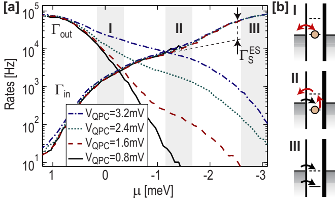
FIG. 4. (Color online) (a) Rates for electrons tunneling into and out of the QD, measured at four cross sections of Fig. 3(b) [position of arrows in Fig. 3(b)]. Only the rate related to absorption ( \Gamma_{\text{out}} ) is strongly influenced by the increase in QPC bias. (b) Energy level diagrams for the three configurations marked in (a).
