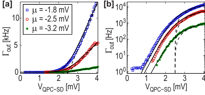
FIG. 5. (Color online) (a) Electron tunneling due to photon absorption, measured versus QPC bias voltage. The data was taken at three different positions of the shoulder seen in Fig. 3. As soon as the QPC bias voltage exceeds the QD level separation \Delta E , the absorption rate increases linearly with V_{\text{QPC}} . (b) Same data as in (a), but plotted in logarithmic scale. The absorption rate shows exponential decay for eV_{\text{QPC}} < \Delta E , with the slope of the decay set by the electron temperature in the QPC. The solid lines are fits to Eq. (6) in the text, while the dashed lines are the corresponding results assuming zero temperature.
